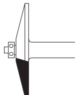
HW RAISED PANEL BITS WITH BALL BEARING GUIDE Z=2 Page 2.24
