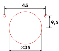
TRIMATIC SUPER 48/6 for hinges type "Salice"
