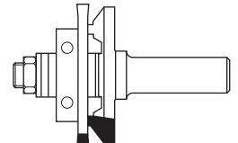
HW V PANELING ASSEMBLY WITH BALL BEARING GUIDE Z=2 Page 2.28
