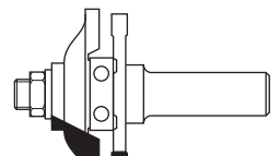
HW STILE AND RAIL ASSEMBLY WITH BALL BEARING GUIDE Z=2 Page 2.30
