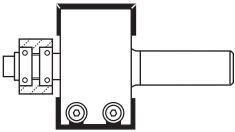
HW INSERT REBATE BITS Z=2 Page 9.20
