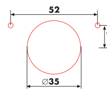
TRIMATIC SUPER 52/7,5 hinges for large thickness
